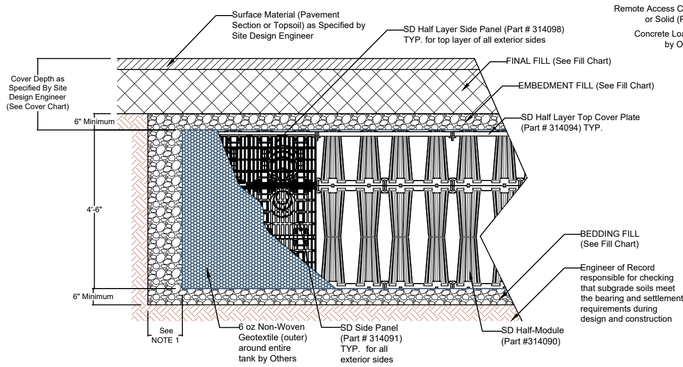
1.5 LAYER SD INFILTRATION CROSS SECTION NTS
