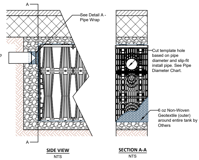
1.5 LAYER SD PIPE INSTALLATION NTS
