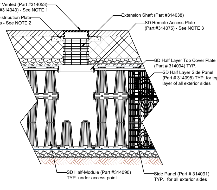
1.5 LAYER SD ACCESS POINT CROSS SECTION NTS
