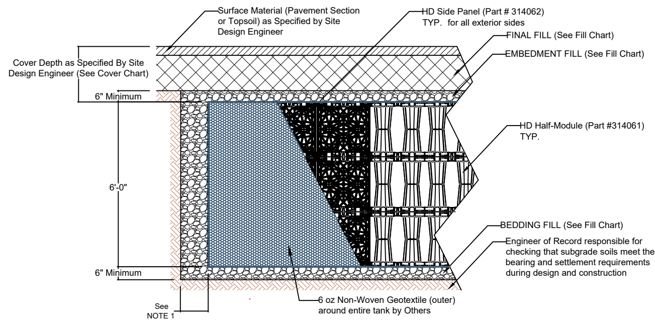
3 LAYER HD INFILTRATION CROSS SECTION NTS
