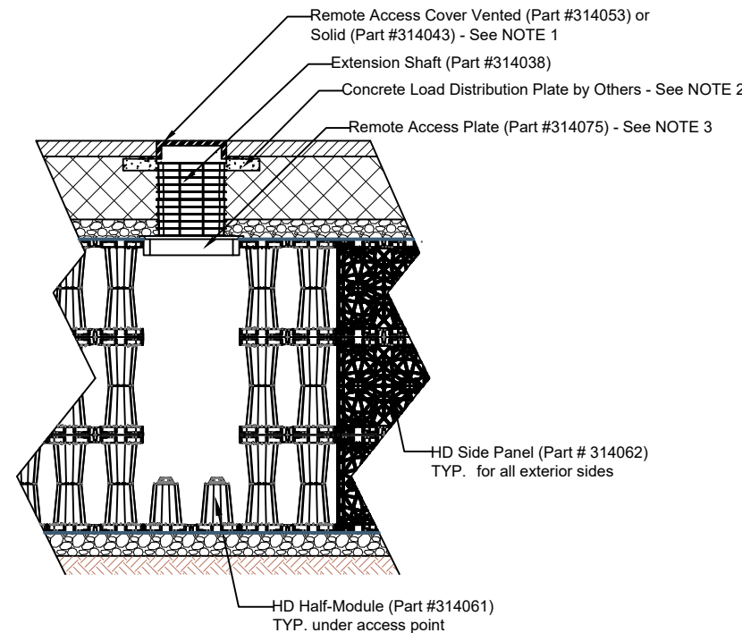
3 LAYER HD ACCESS POINT CROSS SECTION NTS
