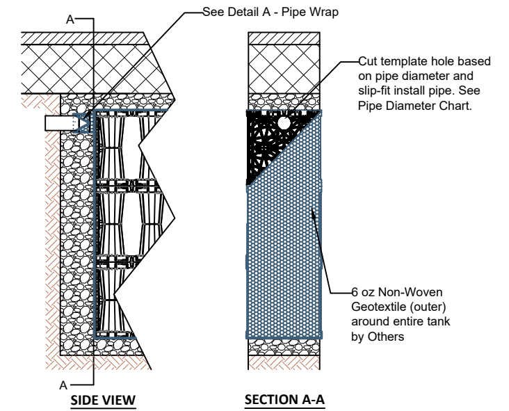
3 LAYER HD PIPE INSTALLATION NTS
