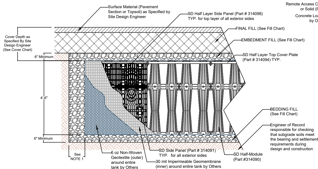
1.5 LAYER SD DETENTION CROSS SECTION NTS
