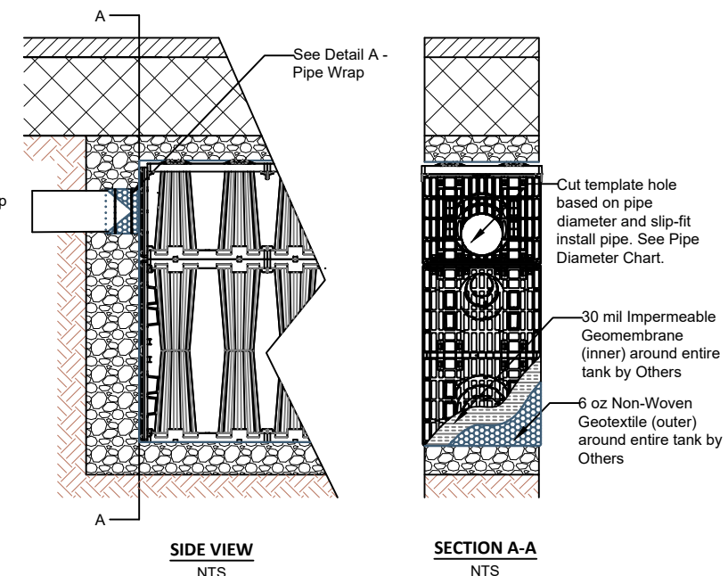
1.5 LAYER SD PIPE INSTALLATION NTS
