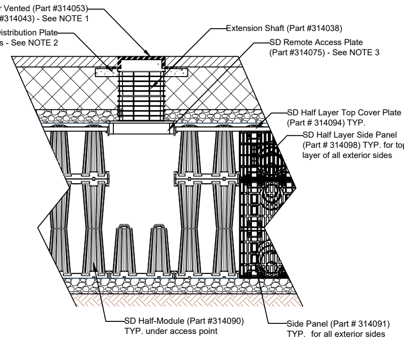
1.5 LAYER SD ACCESS POINT CROSS SECTION NTS
