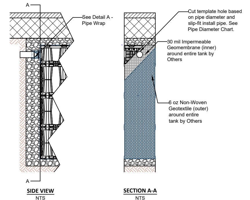
3.5 LAYER HD PIPE INSTALLATION NTS
