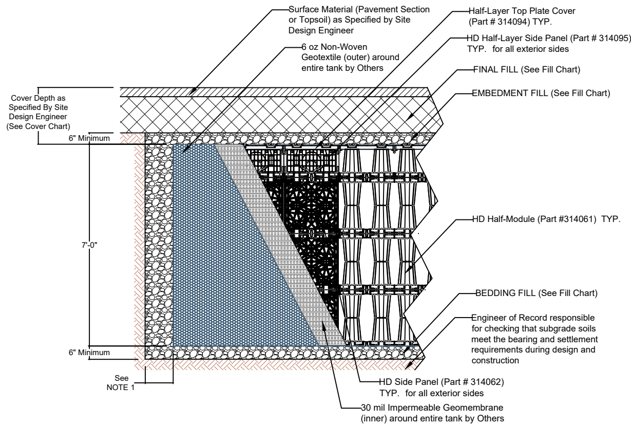
3.5 LAYER HD DETENTION CROSS SECTION NTS
