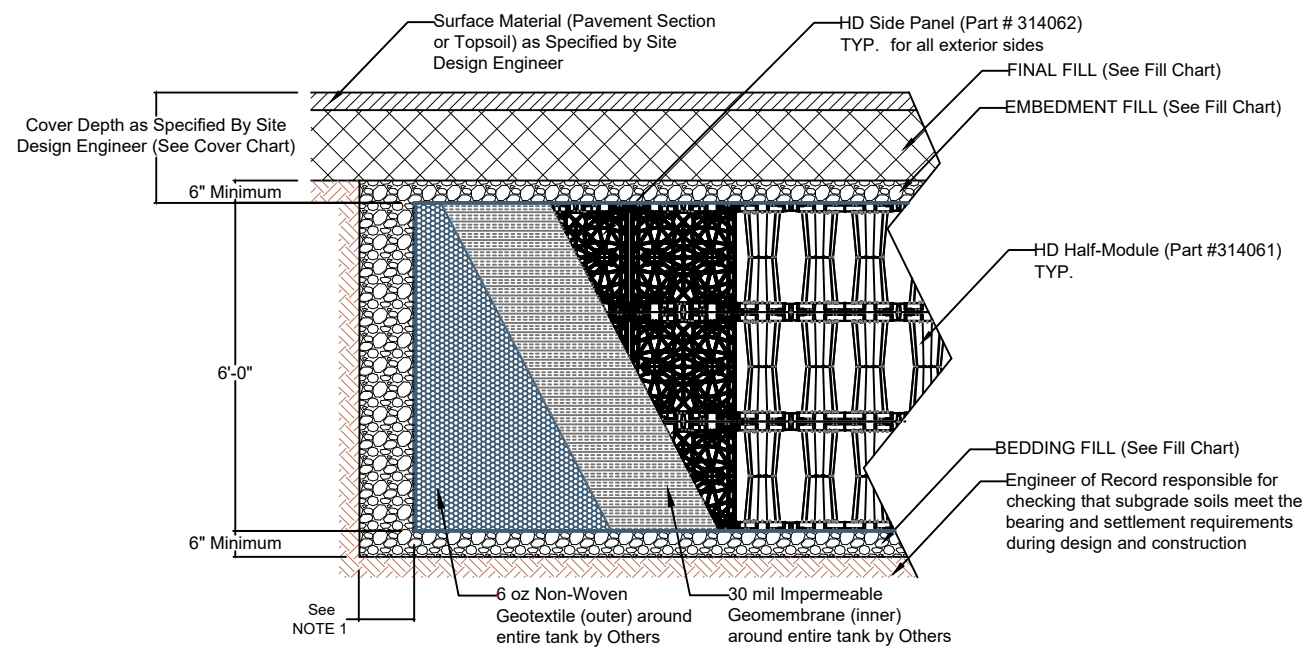
3 LAYER HD DETENTION CROSS SECTION NTS
