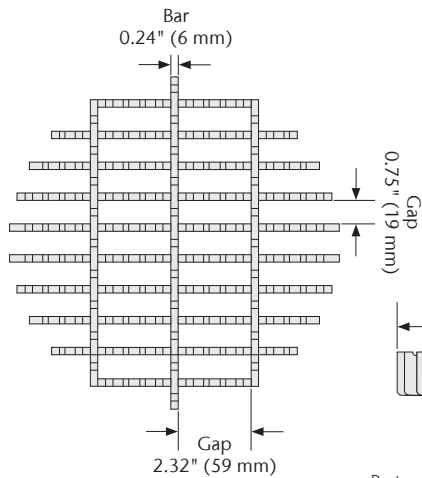
12" Round Frameless Ladder Grate - R50
