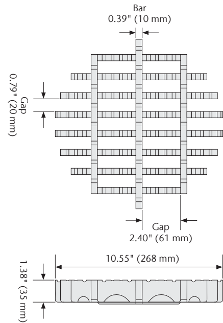
12" Round Frameless Ladder Grate - M125
