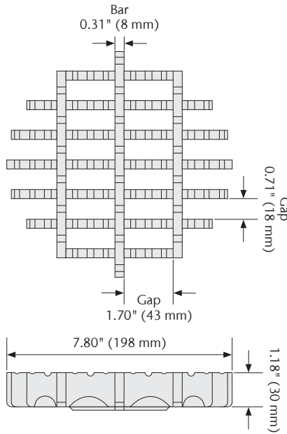
9" Round Frameless Ladder Grate - M125
