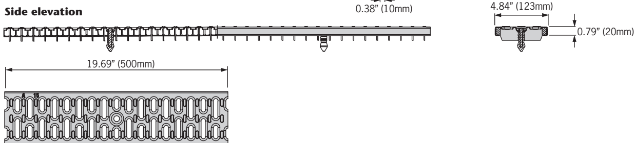
Side elevation
