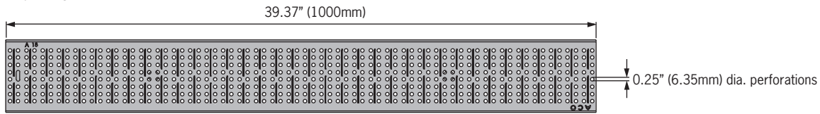
Plan view
