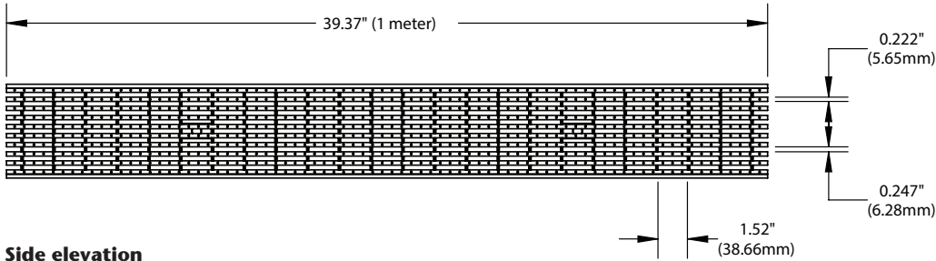
Side elevation
