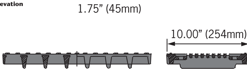
Side elevation
