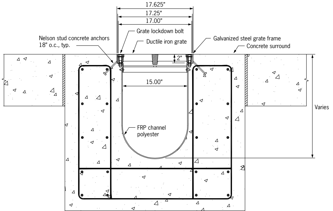
Aquaduct 15" Custom Trench Drain (NTS)
