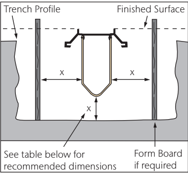
Concrete Surround Dimensions* (x)
