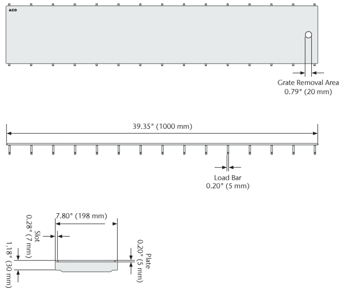
MD Slot Cover Grate - 1000mm
