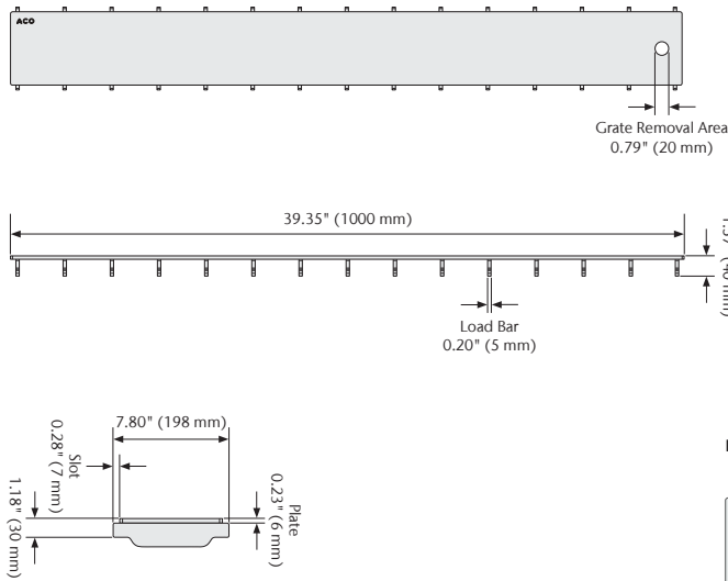
HD Slot Cover Grate - 1000mm
