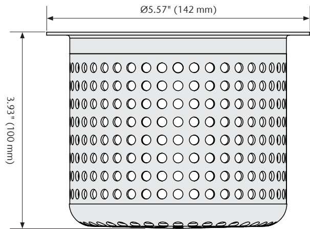
H4.0" Debris Strainer Basket
