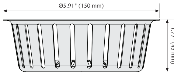
H1.8" Debris Strainer Basket
