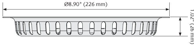
H1.0" Debris Strainer Basket
