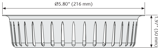
H2.0" Debris Strainer Basket
