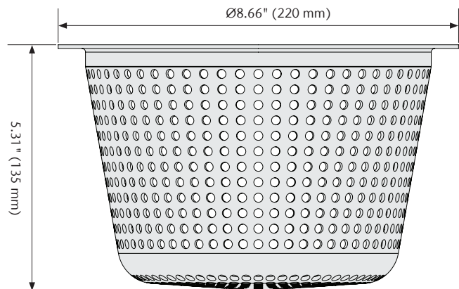
H5.3" Debris Strainer Basket
