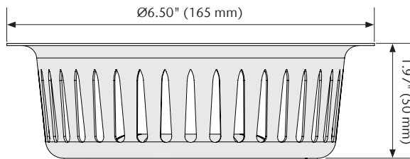
H2.0" Debris Strainer Basket
