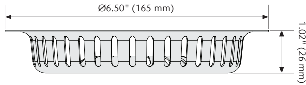
H1.0" Debris Strainer Basket
