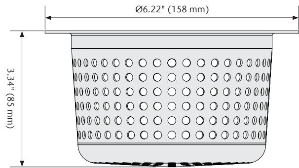
H3.3" Debris Strainer Basket
