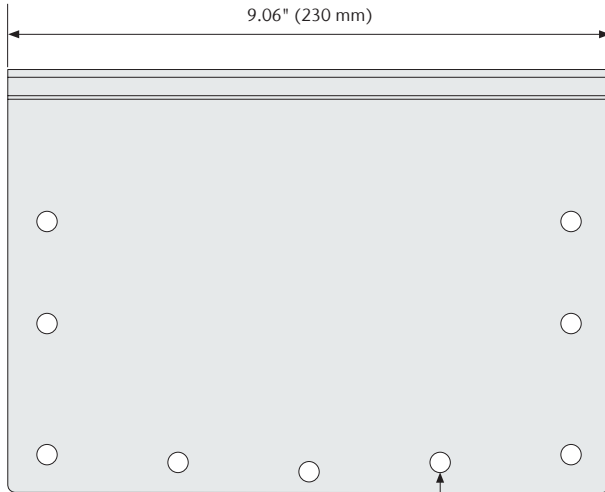
Ø0.28" (7 mm) Thru Holes For M6 Connection Bolts
