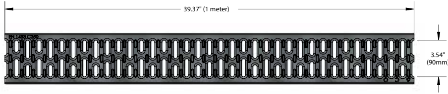
Plan view
